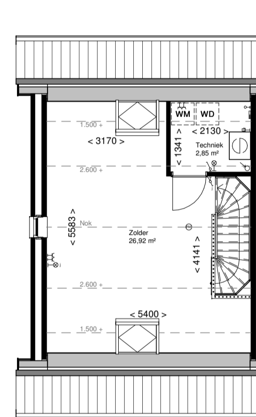
R 502 Dakraam ca. 1140x1180mm in hellend dak
